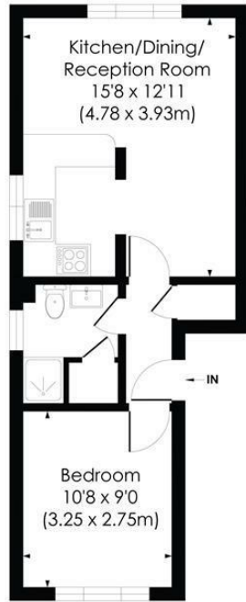
THIRD FLOOR
